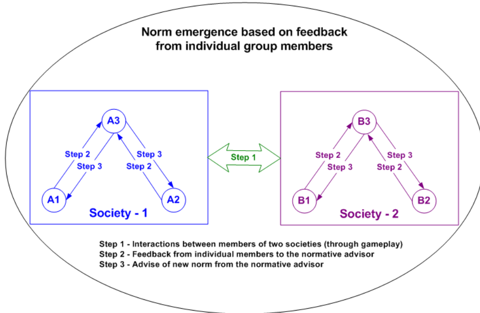
Figure 1: Architecture of collective individual feedback mechanism for norm emergence
